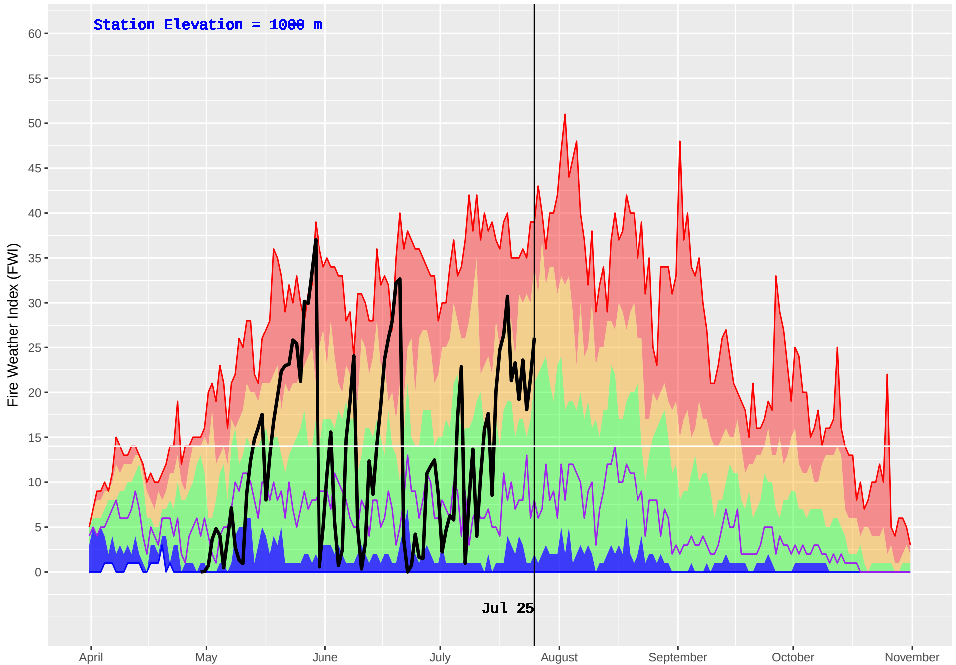
SUCCOUR CREEK (374) : Historical (1986–2016) and Current (2018) Noon Fire Weather Index (FWI)
